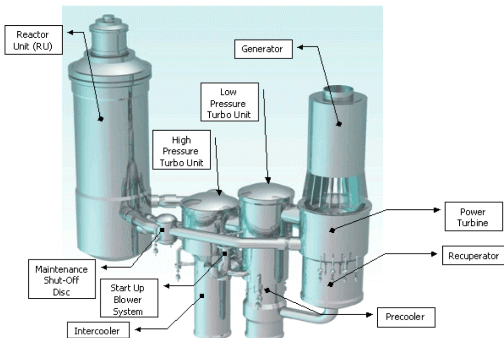
Figure 2. PBMR pressure boundary
