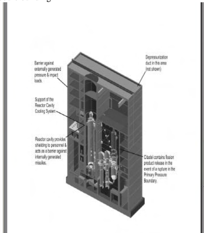
Figure 5. PBMR single module building
