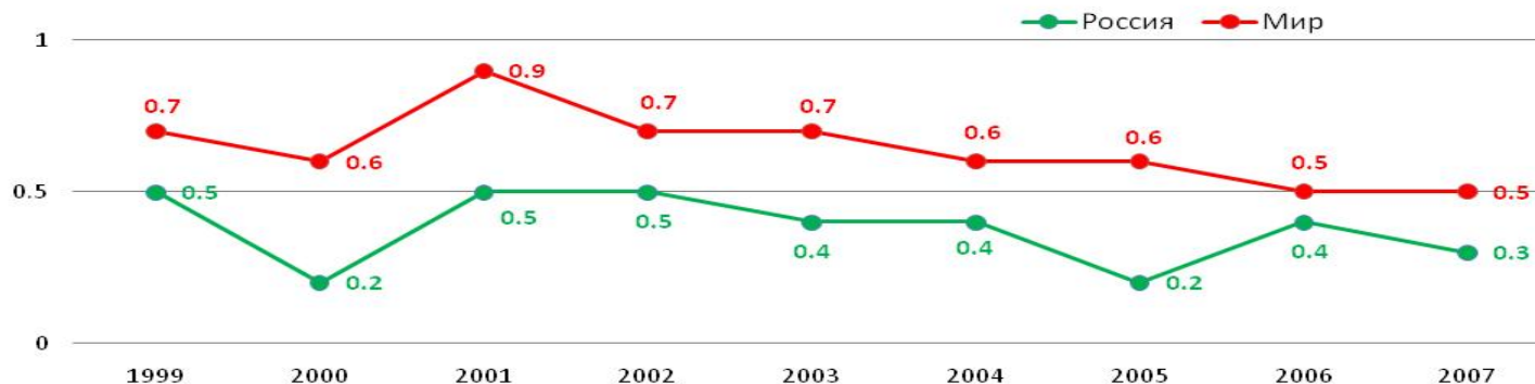
Automatic shut downs from criticality World average and Russia (WANO data)
